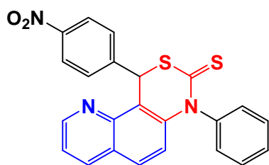
Structure of Compound HQNO2
